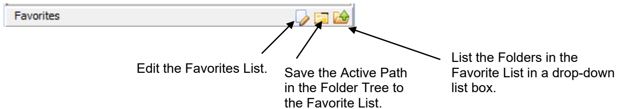
Figure 2.7 Favorites Bar
