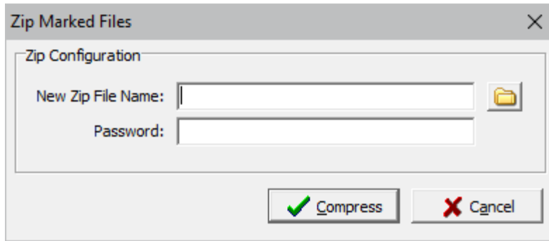
Figure 2.12 Zip Dialog
