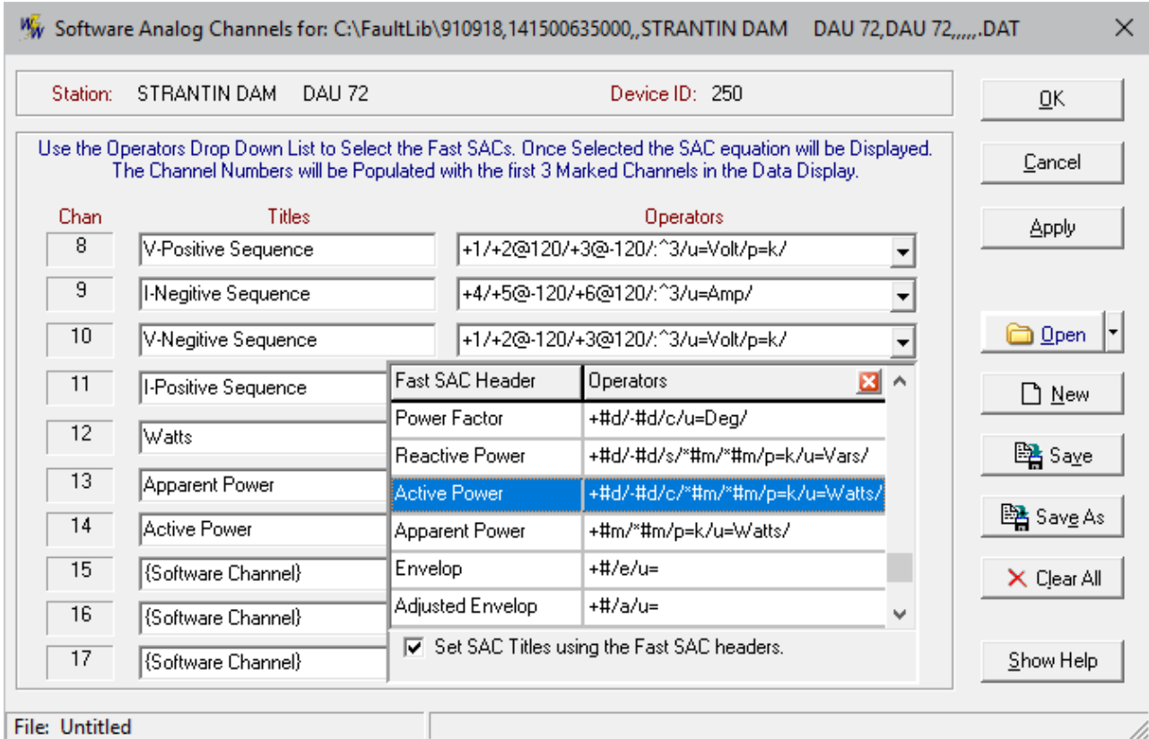
Figure 3.42 SAC Dialog
