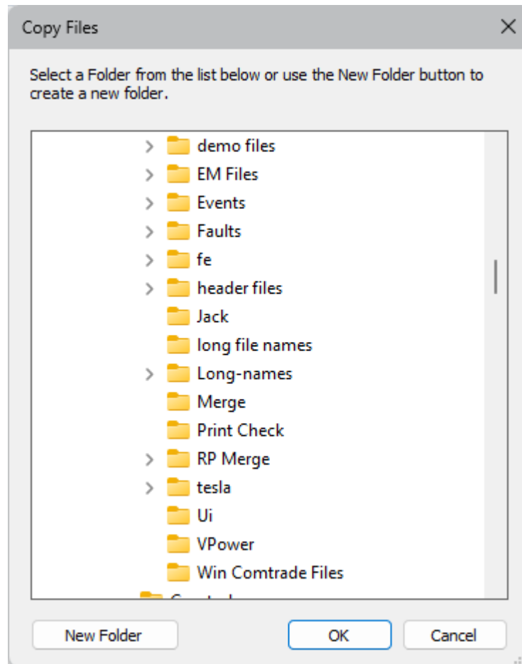
Figure 2.10 Copy Dialog
