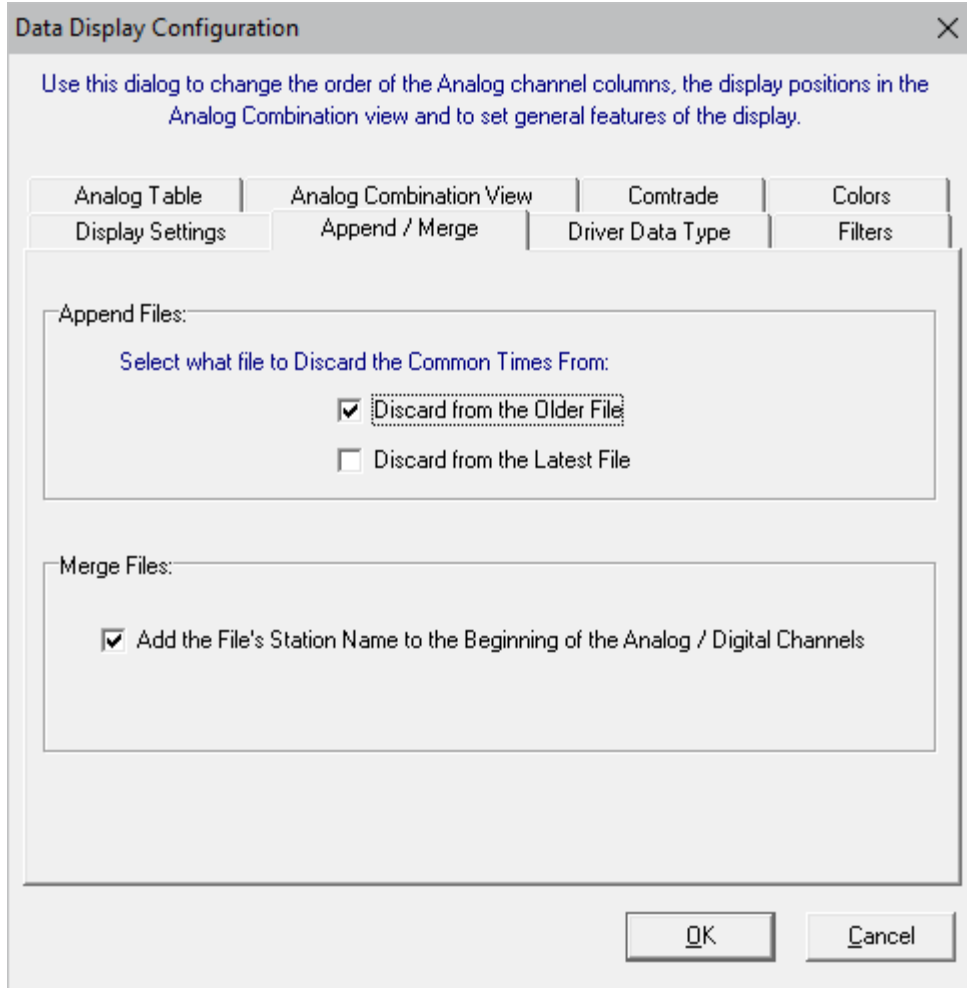
Figure 2.25 Append/Merge Properties
